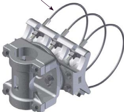
AB-0336/ AB-0337 Cable Kit
