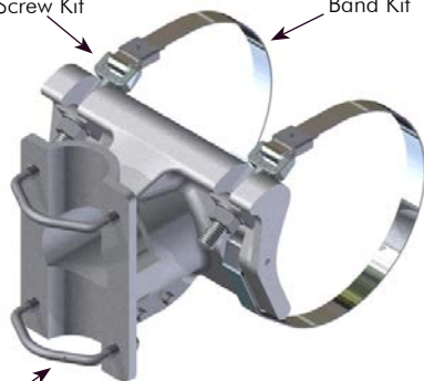
AB-0243 Band Kit
