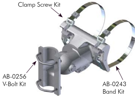
AB-0204 Clamp Screw Kit
