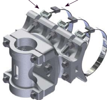
AB-0303 Clamp Screw Kit
