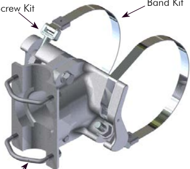
AB-0243 Band Kit
