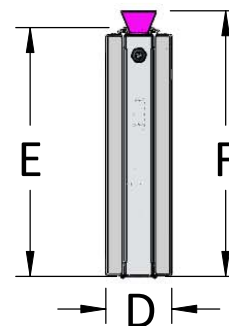
Right Side View With Tristud Mount Option (TA)
