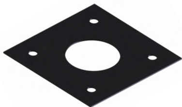
PB-0550-PNC Template, ABS Plastic 13" Bolt Circle for Square and Octagonal Bases
