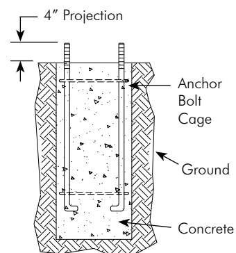
Typical Footing Detail
