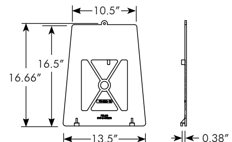
Door Assy, Plastic Flat Short w/ Tab on Top, No Latch
